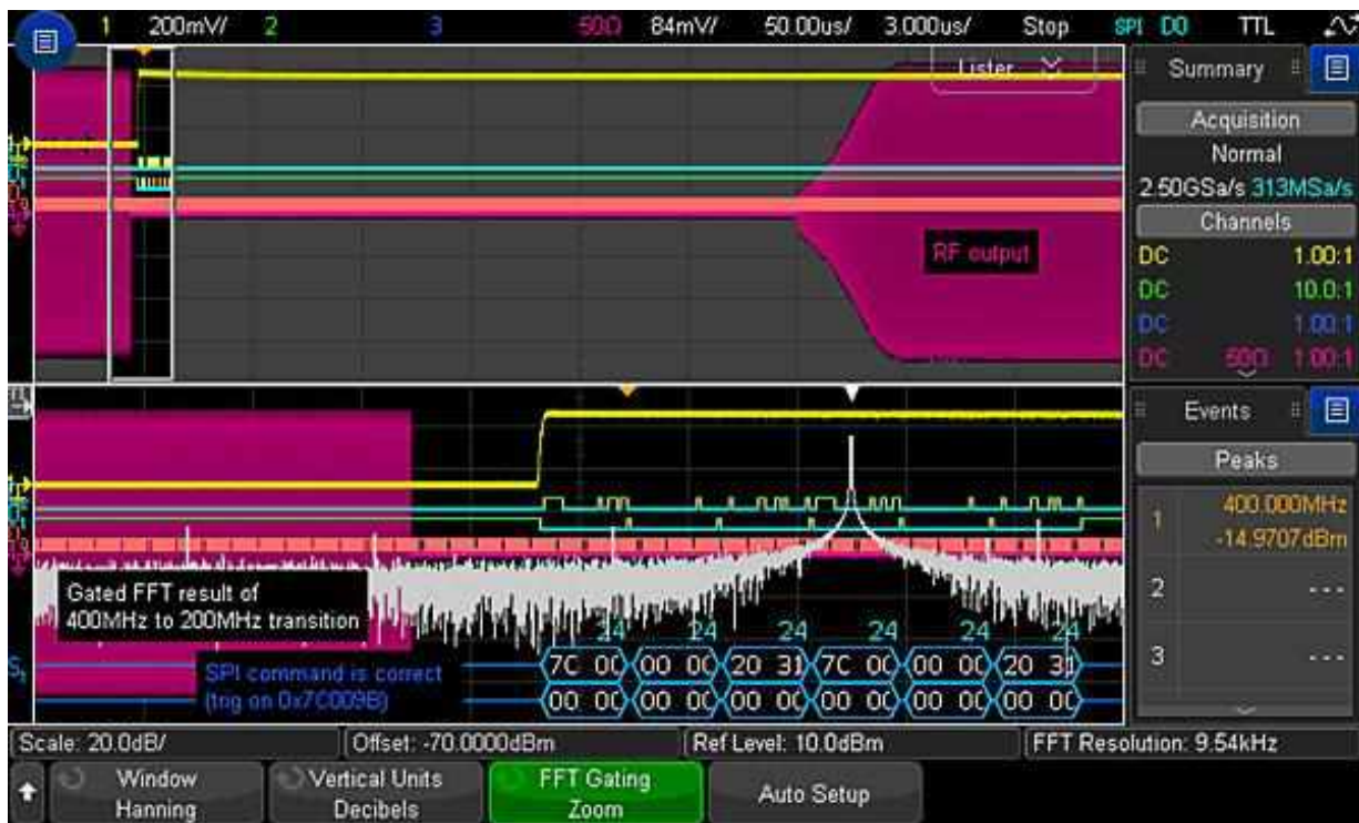
Figure 21. Triggered on a SPI command, the RF signal is still at 400 MHz as indicated in the frequency peak search result lister.
